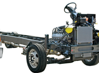
F-59 Commercial Stripped Chassis
